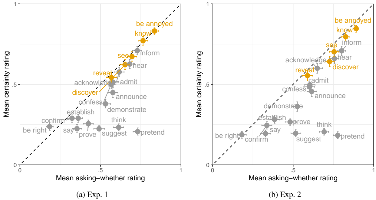
Figure A10: By-predicate mean projection against mean at-issuence. Purportedly factive predicates in orange. Error bars indicate 95% bootstrapped confidence intervals.
