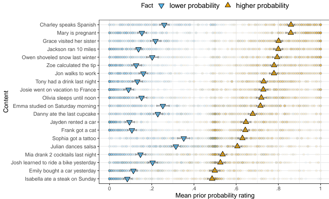
Figure A1: Mean prior probability rating by content and fact in Exp. 1. Error bars indicate 95% bootstrapped confidence intervals. Transparent dots indicate individual participant ratings.
