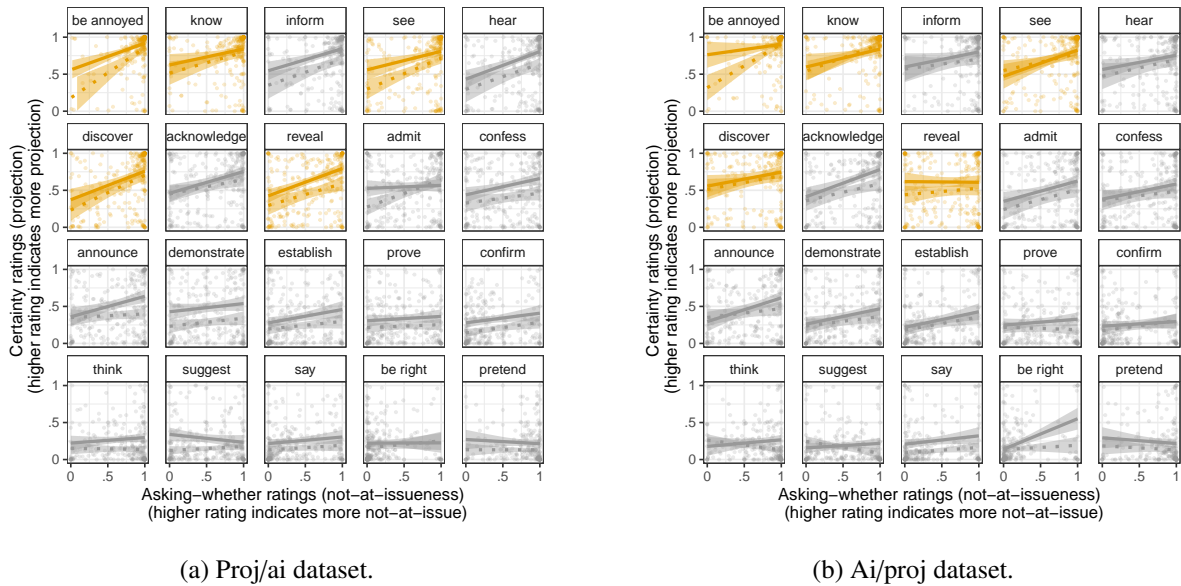
Figure A8: Participants' certainty ratings (measuring projection) against asking-whether ratings (measuring at-issuence) by high (solid line: —) and low prior probability fact (dotted line: ···) in Exp. 1: (a) Proj/ai dataset, (b) Ai/proj dataset. Linear smoothers with 95% confidence intervals overlaid Predicates are ordered by projection mean, with purportedly factive predicates in orange.
