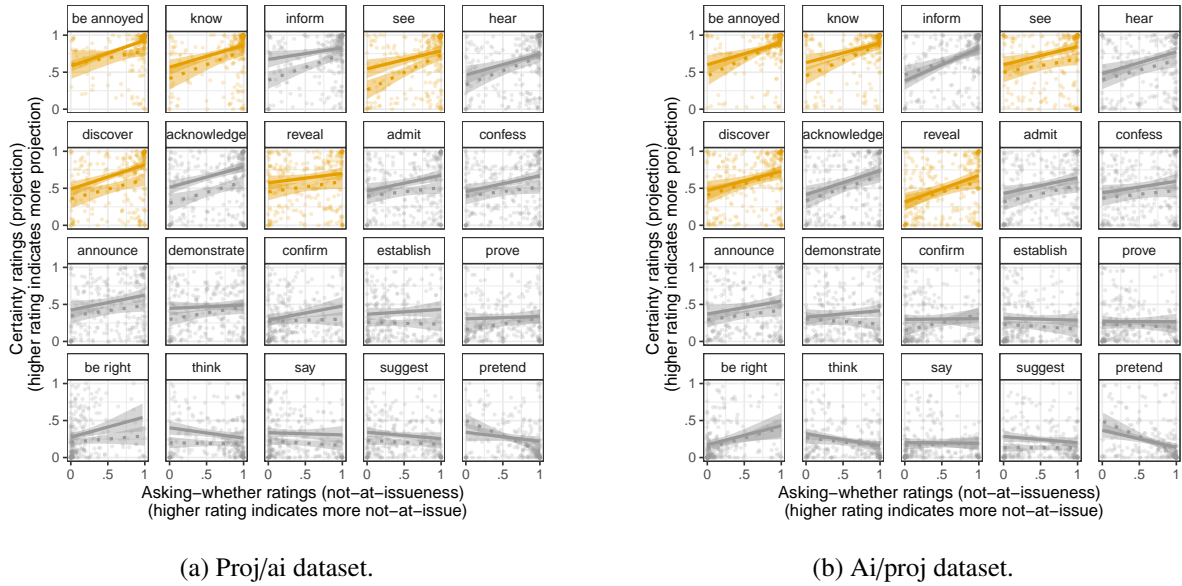
Figure A4: Participants' certainty ratings (measuring projection) against asking-whether ratings (measuring at-issueness) by high (solid line: —) and low prior probability fact (dotted line: ···) in Exp. 1: (a) Proj/ai dataset, (b) Ai/proj dataset. Linear smoothers with 95% confidence intervals overlaid Predicates are ordered by projection mean, with purportedly factive predicates in orange.
